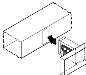
Fig. 2 – Installation drawing of slip-in heater.
