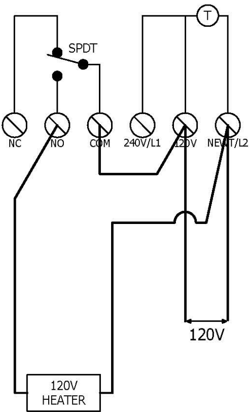
120V WIRING DIAGRAM
