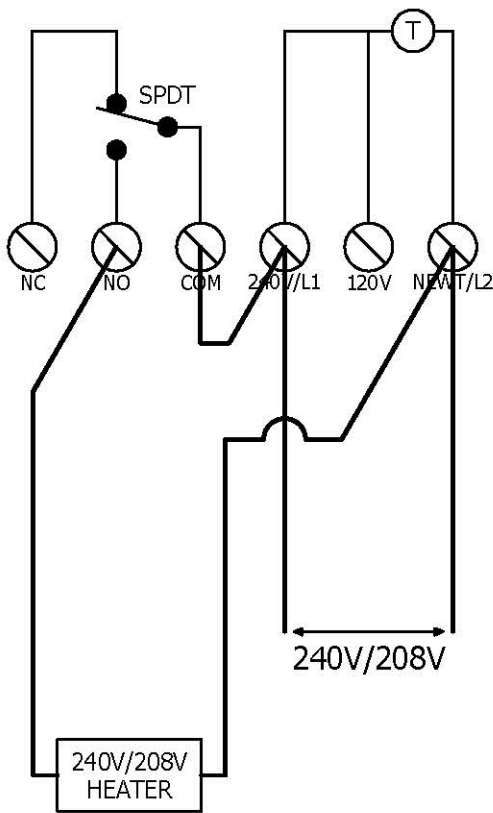
240V / 208V WIRING DIAGRAM
