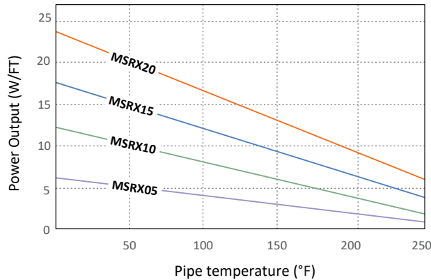
MSRX Power-Temperature Characteristics
