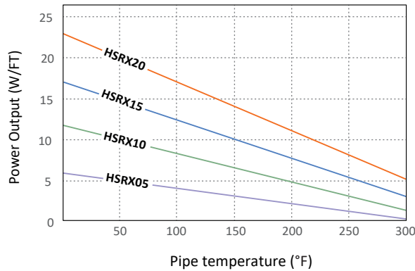
HSRX Power-Temperature Characteristics
