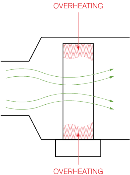
Heater adjacent to transition
