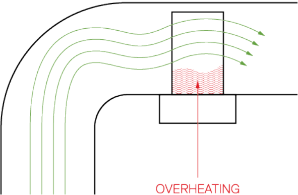
Heater too close to elbow
