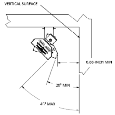
Fig. 5 – CEILING MOUNTING ANGLED AWAY FROM VERTICAL SURFACE
