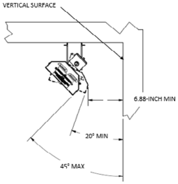
Fig. 5 – CEILING MOUNTING ANGLED AWAY FROM VERTICAL SURFACE
