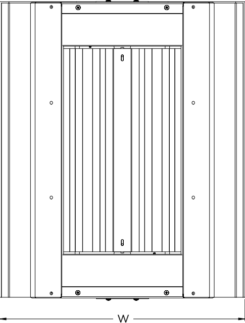
Dimensions: 2-Element
