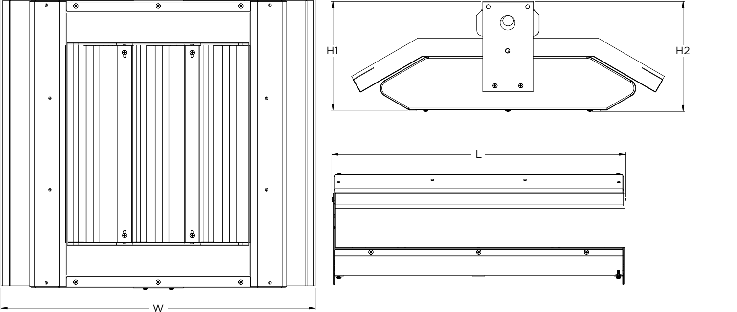
Dimensions: 3-Element
