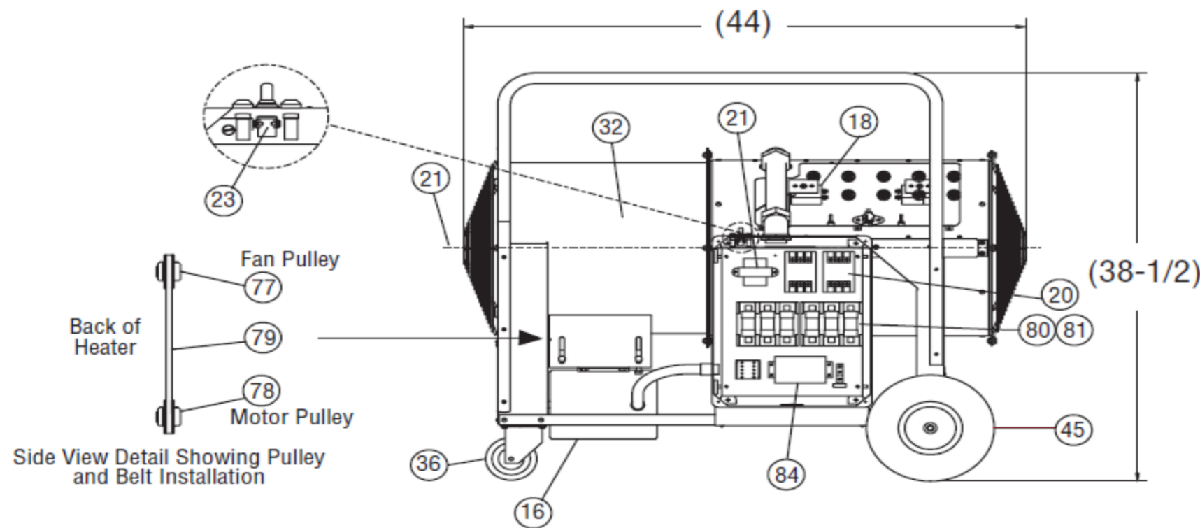
Element Assembly 48kW
