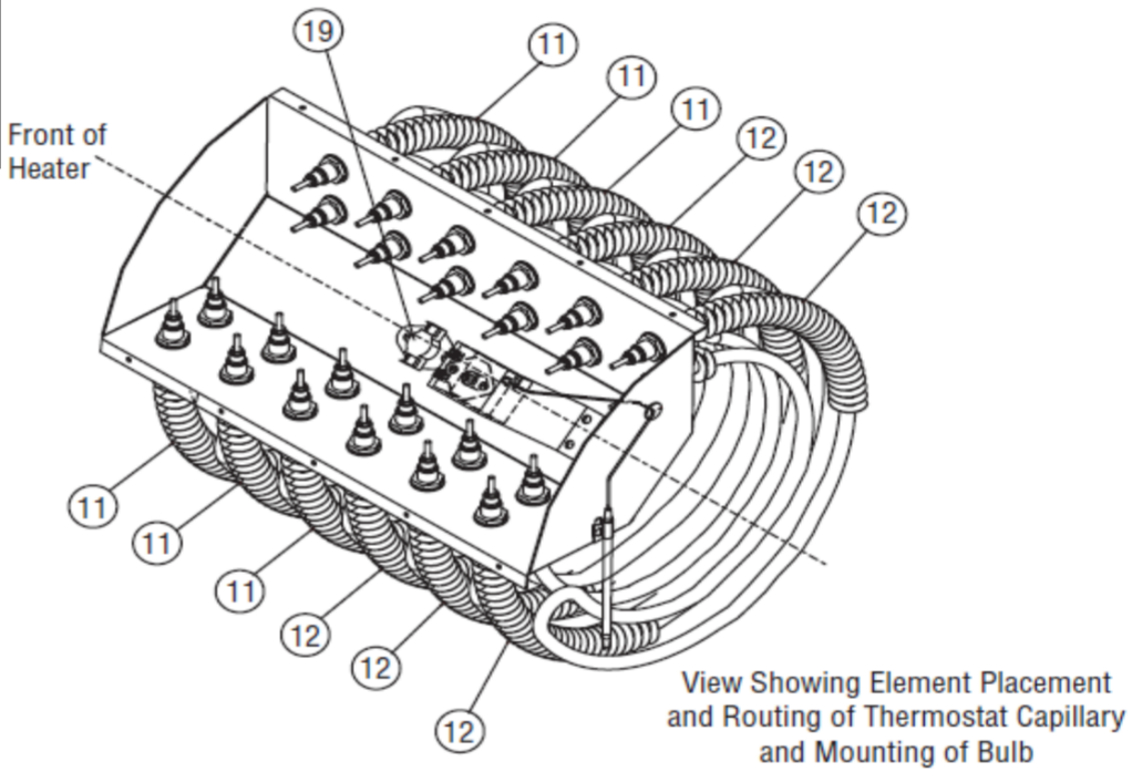
Element Assembly 60kW
