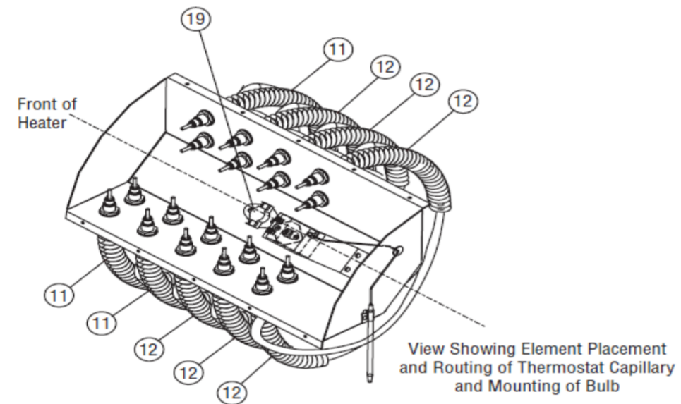
Element Assembly 48kW
