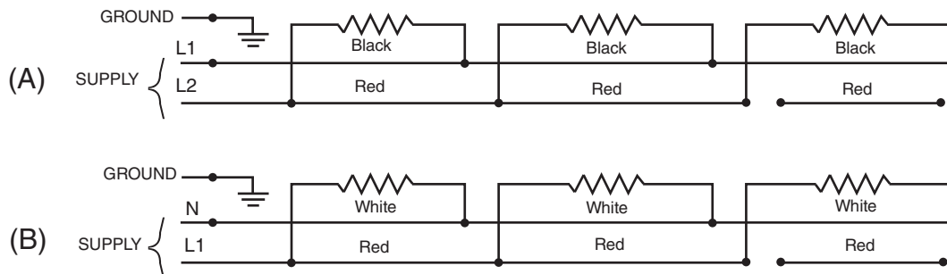
Figure 5. Heater Wiring
