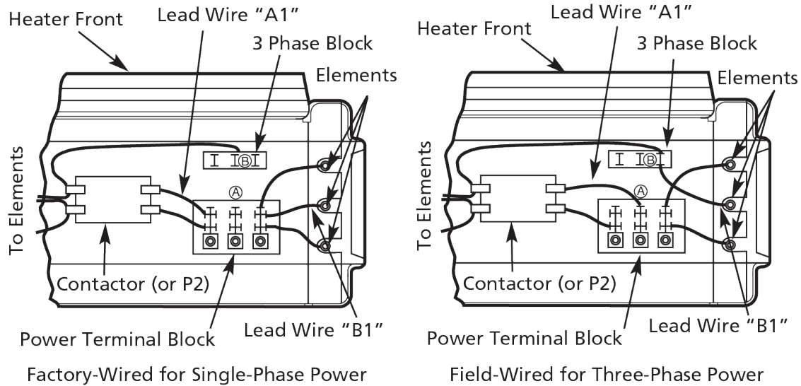
Figure 3a. Wiring Connections for Single-Phase and Three-Phase Power (MUH0321, MUH0521, MUH0581)
