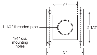
7 IN. HEATER PEDESTAL
