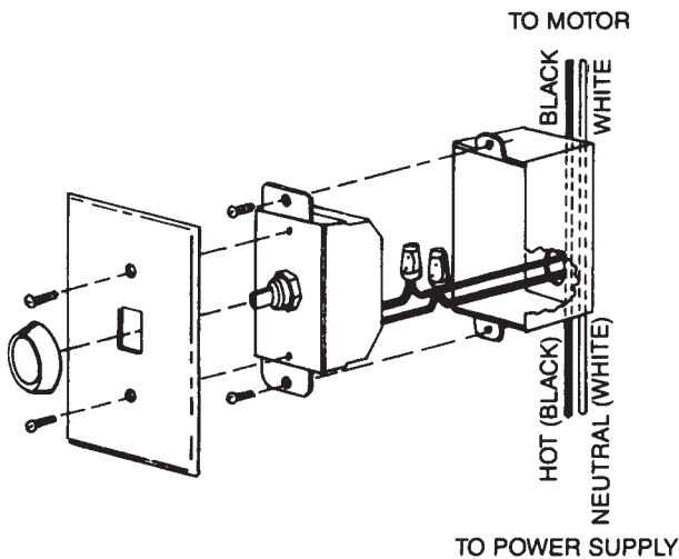
Figure 1 - Mounting Illustration
